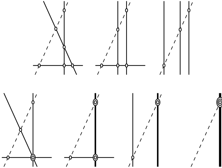
The seven cases of interpolation to data given on three lines in \mathbb{R}^2 .
