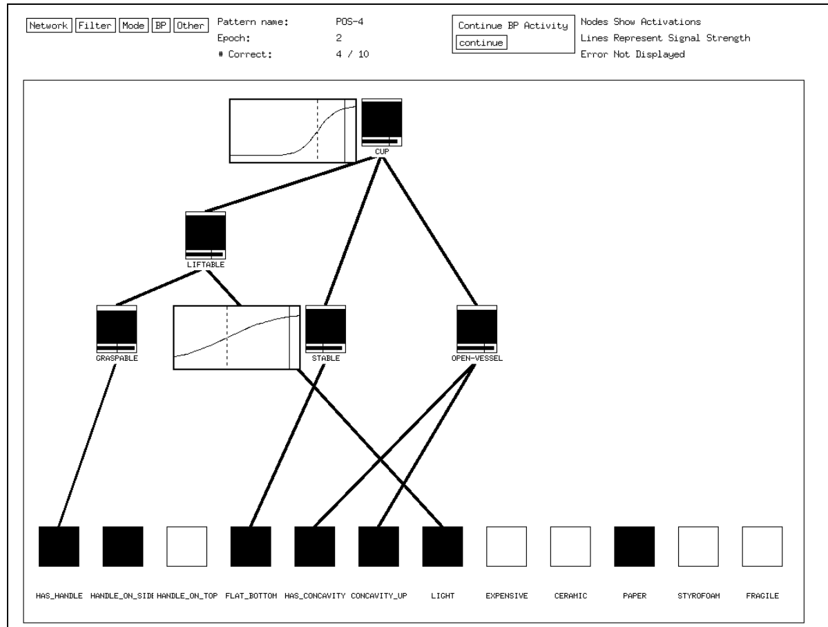
Figure 13: Activation signals and effective activation functions as depicted by Lascaux. The lines connecting units represent forward-propagated signals. The effective activation functions are shown for the STABLE and CUP units.
