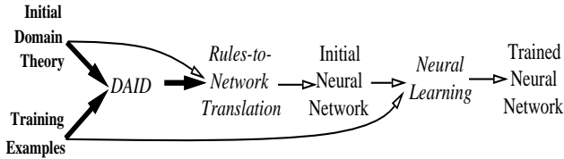
Figure 4: Flow of information using KBANN-DAID.
