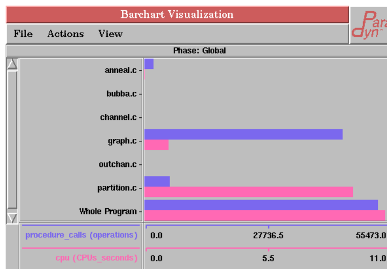
Figure 42: Barchart showing total values
