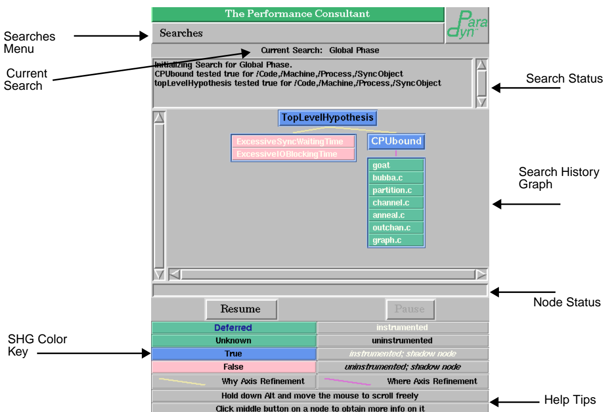
Figure 31: A sample Performance Consultant window
