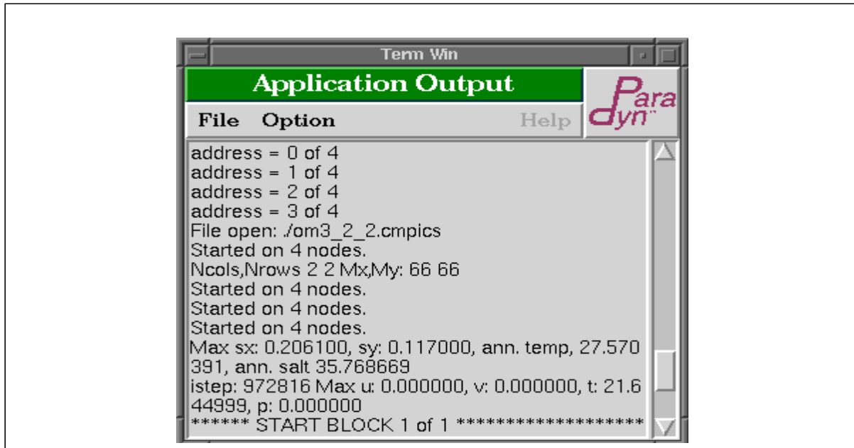
Figure 47: Application output window
