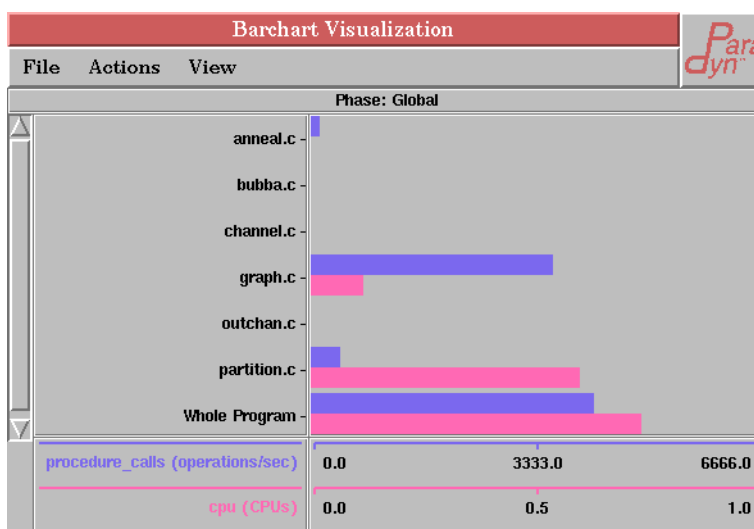
Figure 41: Barchart visualization window
