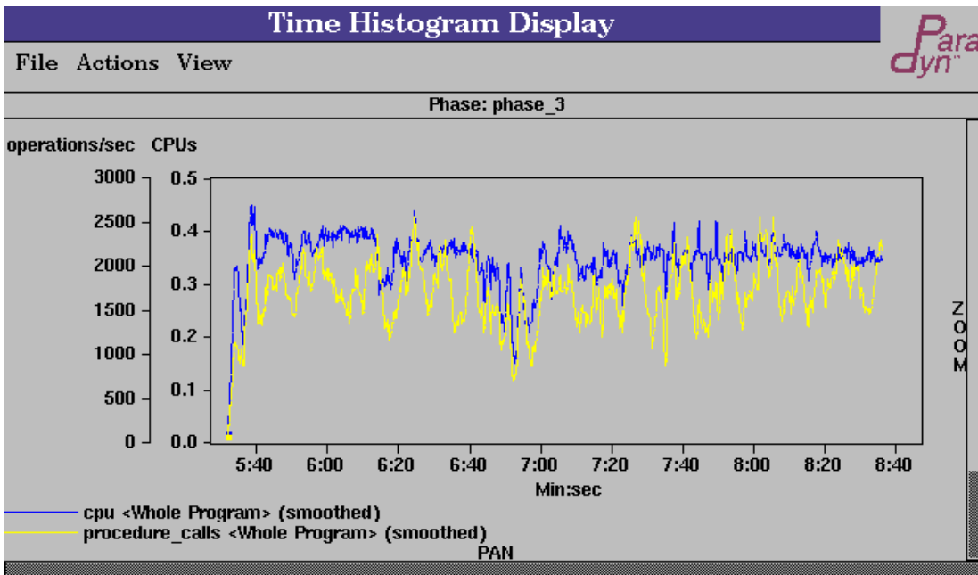
Figure 29: Time Histogram: Local Phase (3)
