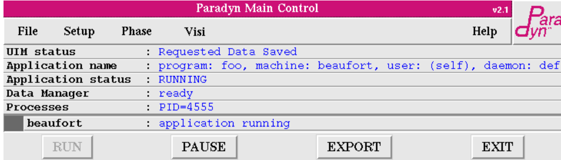
Figure 50: The Paradyn Main Window after saving performance data.
