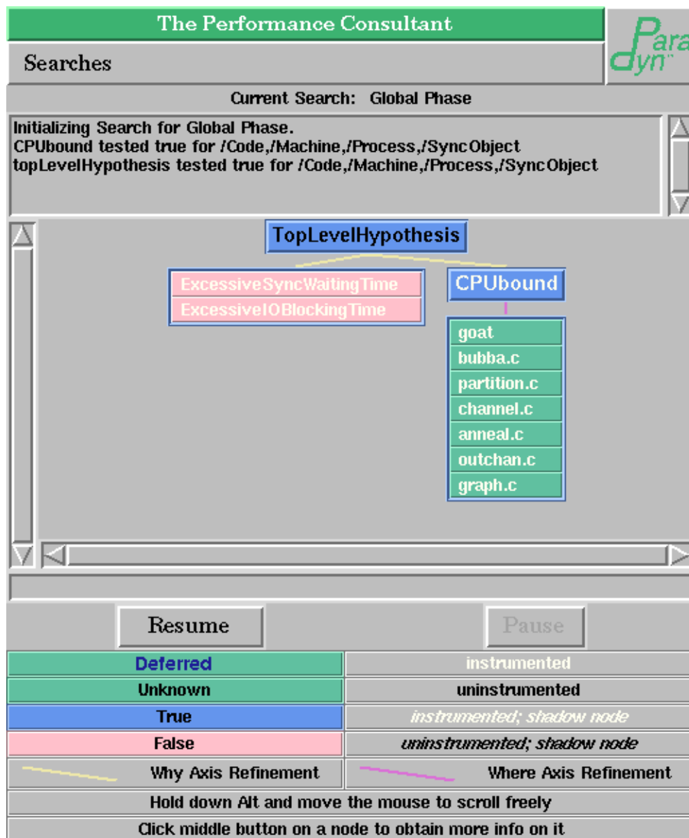
Figure 33: The Performance Consultant refines bottleneck to CPUbound
