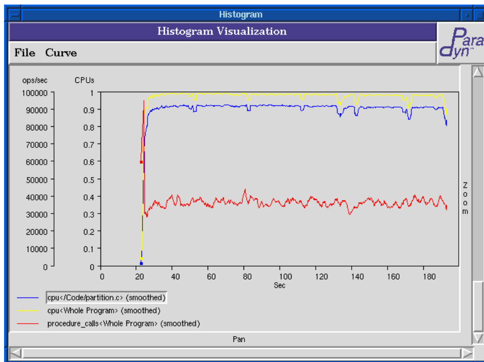
Figure 38: Time Histogram with selected curve
