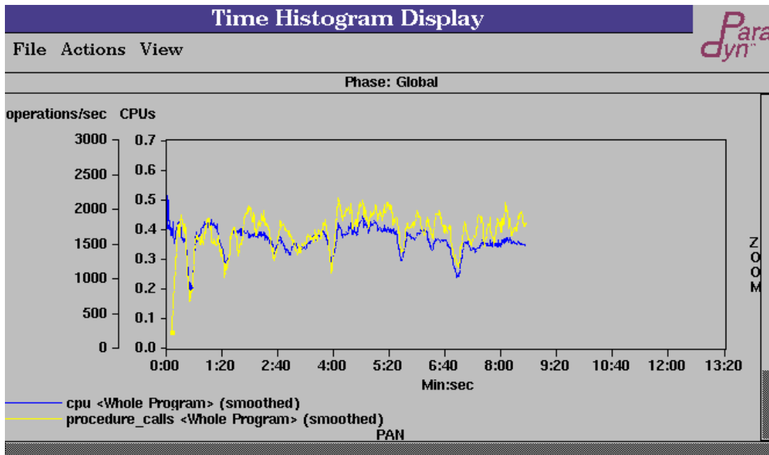
Figure 28: Time Histogram: Global Phase
