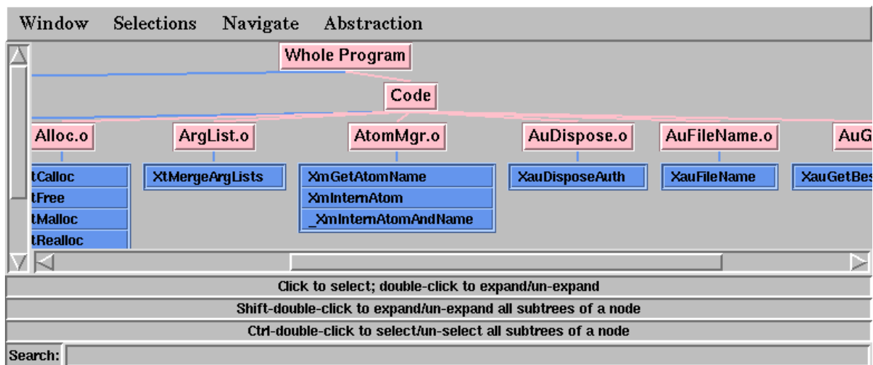
Figure 16: Showing all resources in the Where Axis display
