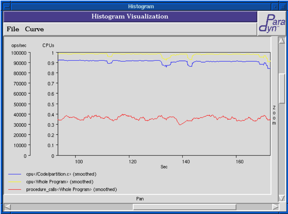
Figure 40: Zoomed Time Histogram
