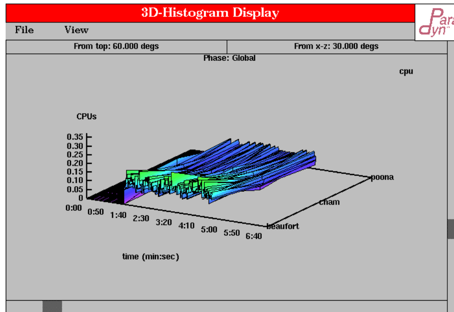
Figure 46: 3D Terrain visualization
