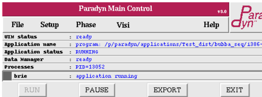
Figure 8: Attach completed and application execution continuing.
