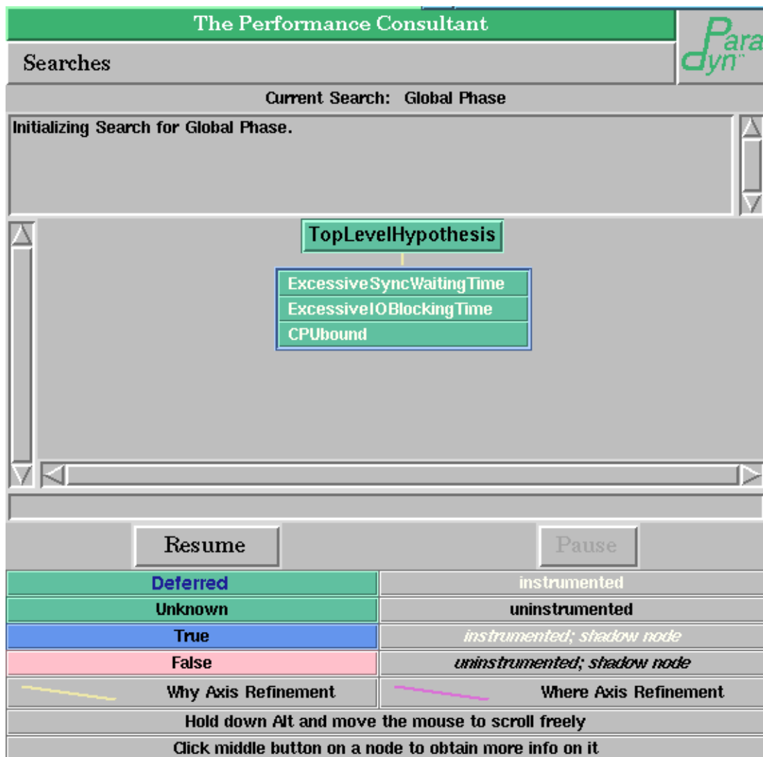
Figure 32: The Performance Consultant's search begins
