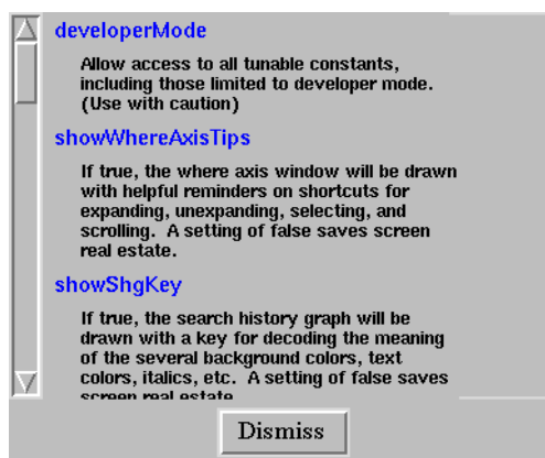
Figure 12: Tunable Constants Descriptions Window
