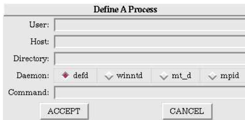
Figure 5: Defining a new application process
