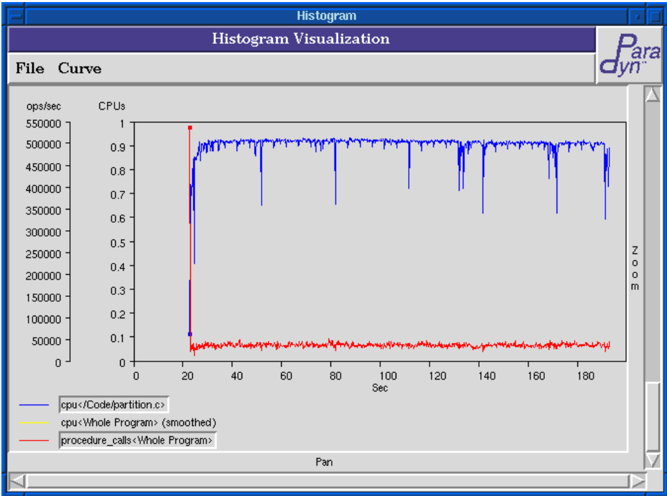
Figure 39: Time Histogram with unsmoothed and hidden curves
