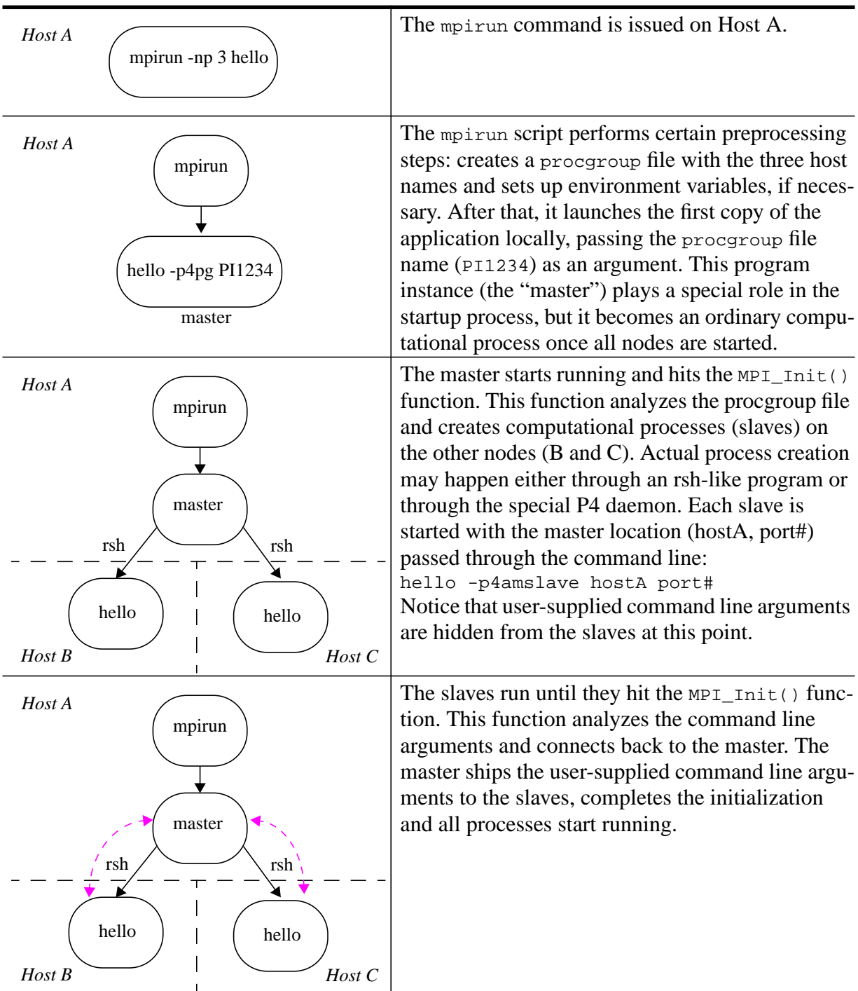
Figure 16: MPICH Job Launch Procedure
