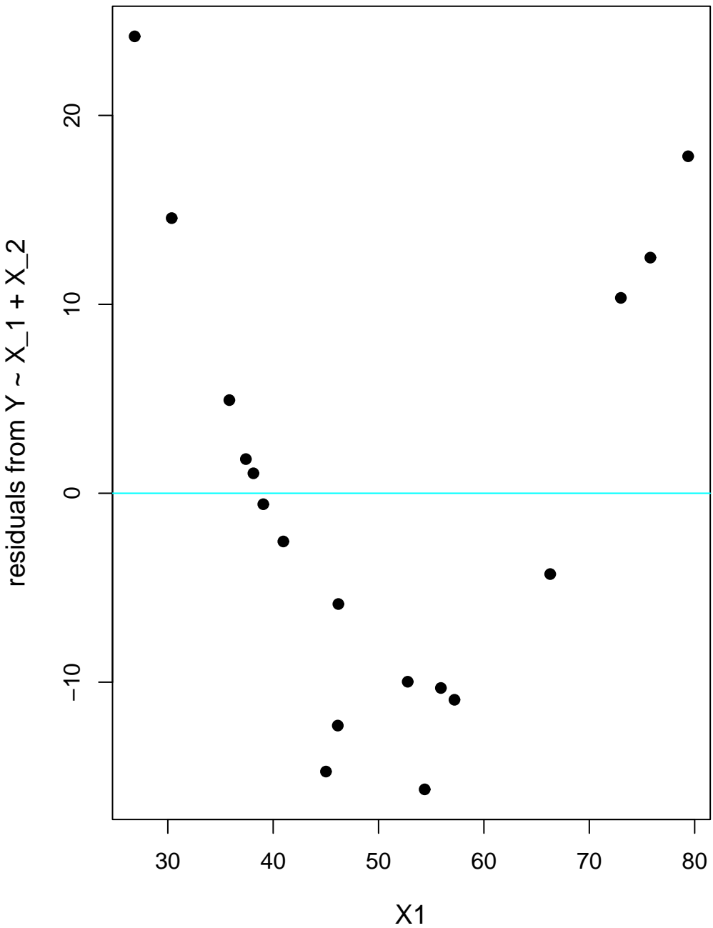
Residual plot against X1
