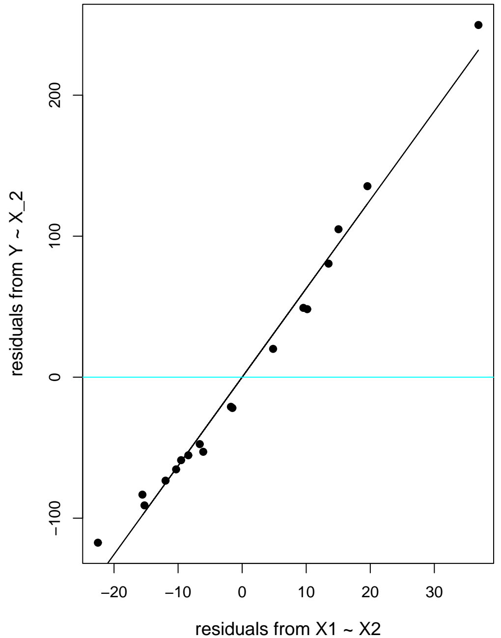
Added-variable plot for X1
