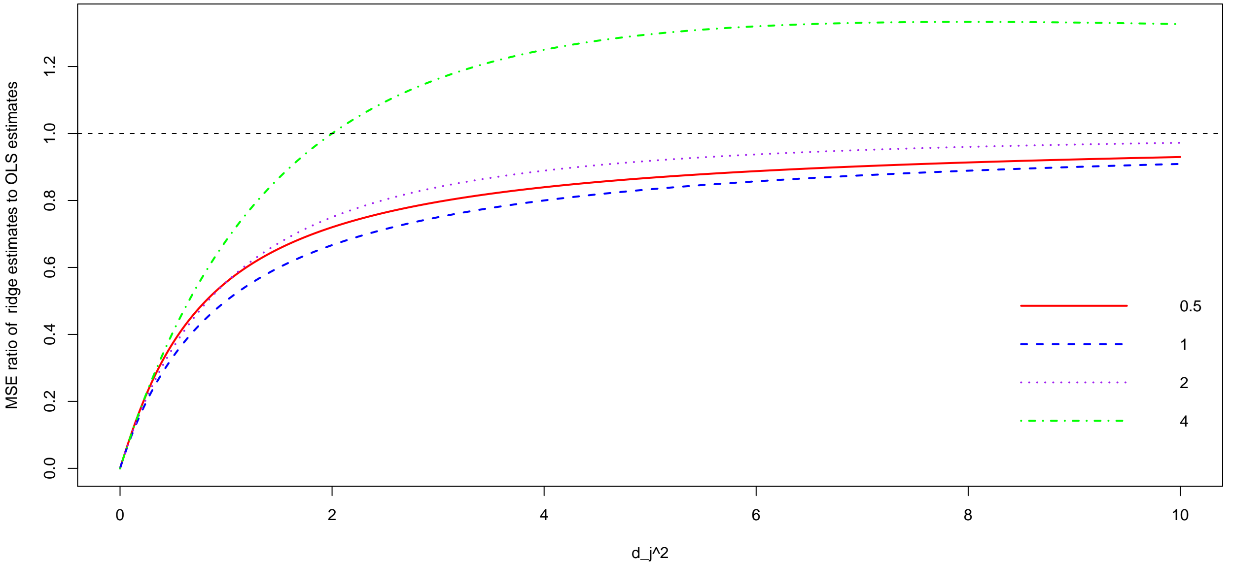
MSE(Beta_Ridge)/MSE(Beta_OLS)
