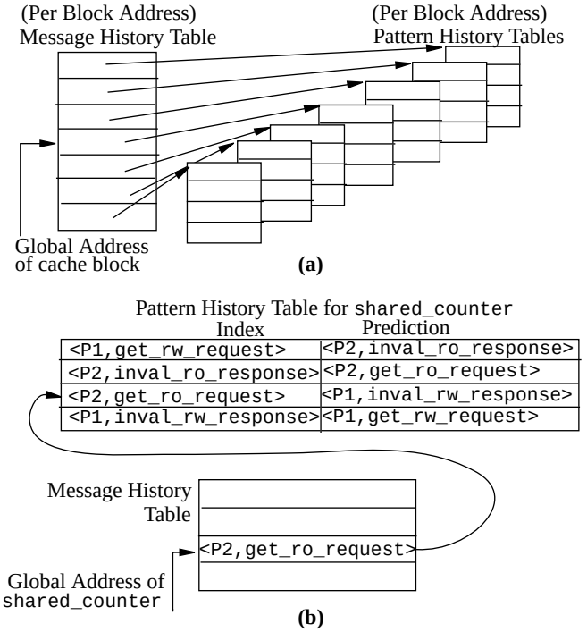
FIGURE 3. (a) shows the logical structure of the Cosmos coherence message predictor and (b) shows an example of how the message and pattern history tables for a directory may look like for the shared_counter in Figure 2. In this example, we assume that the last message received by the directory is a get_ro_request from the consumer (denoted as P2). So, Cosmos will predict the next message to be an inval_rw_response from the producer (denoted as P1).
