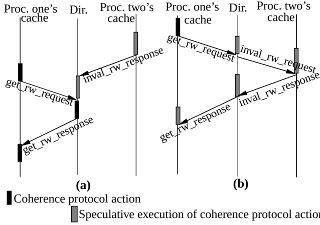
FIGURE 4. Two examples of using prediction to accelerate coherence protocols. (a) shows a protocol in which protocol actions are accelerated in anticipation of processor one's write miss. (b) shows a protocol that predicts incoming coherence messages, updates protocol state, generates (but does not send) messages speculatively, and commits protocol state and messages only if the predicted message arrives. Dir. = Directory, Proc. = Processor. Section 4 outlines possible triggers for the speculative actions shown in this figure.
