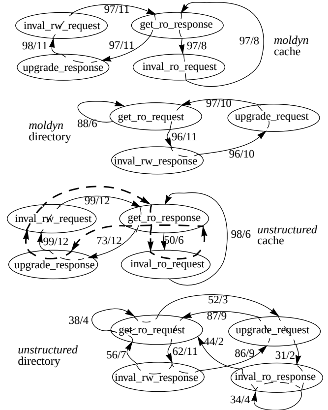
FIGURE 7. Dominant (incoming) message signatures for moldyn and unstructured . See caption of Figure 6 for an explanation of the figure. We show unstructured 's second dominant message signature (at the cache) using bold and dashed lines.
