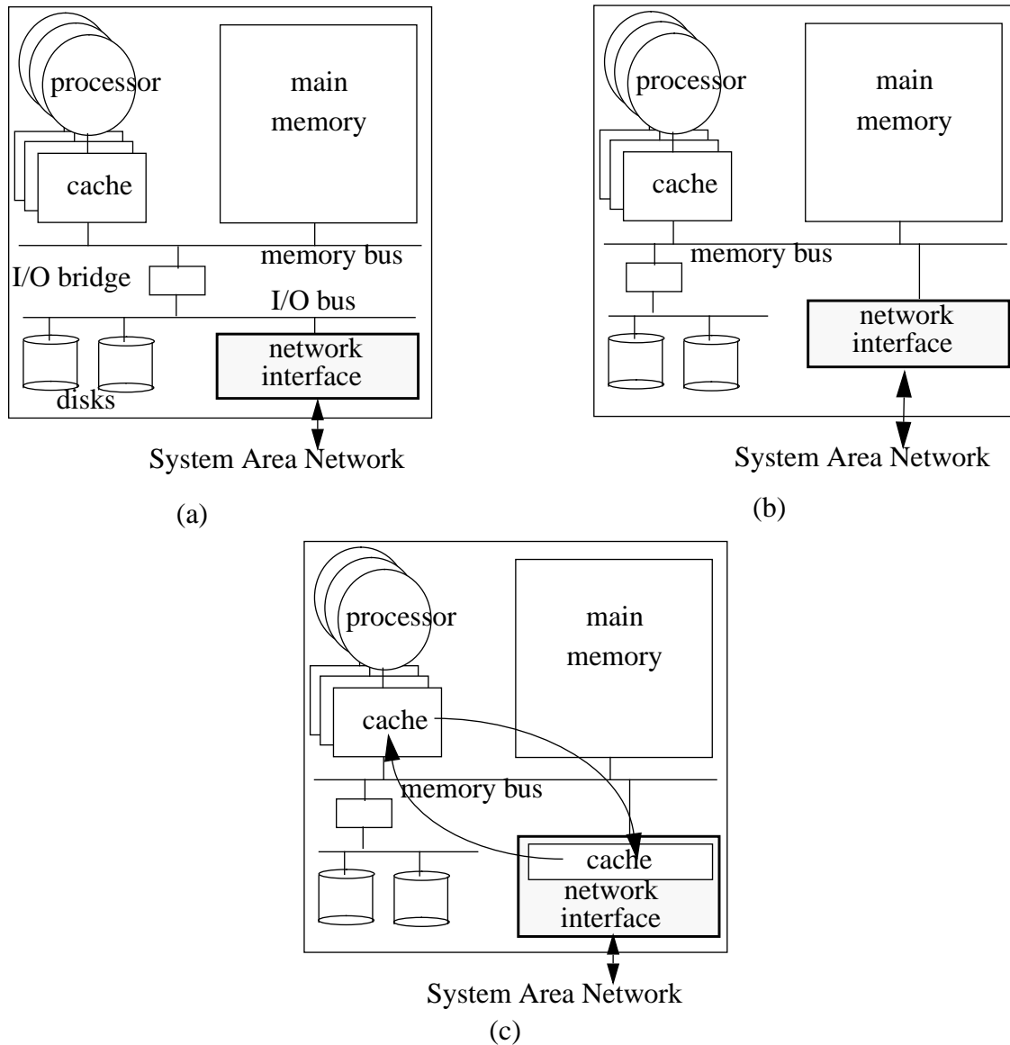
Figure 2-1. Workstation Nodes with Network Interfaces. (a) shows the architecture of standard workstation node with the network interface on the I/O bus. (b) shows the same workstation node with the network interface on the memory bus. (c) augments the network interface in (b) with a cache.
