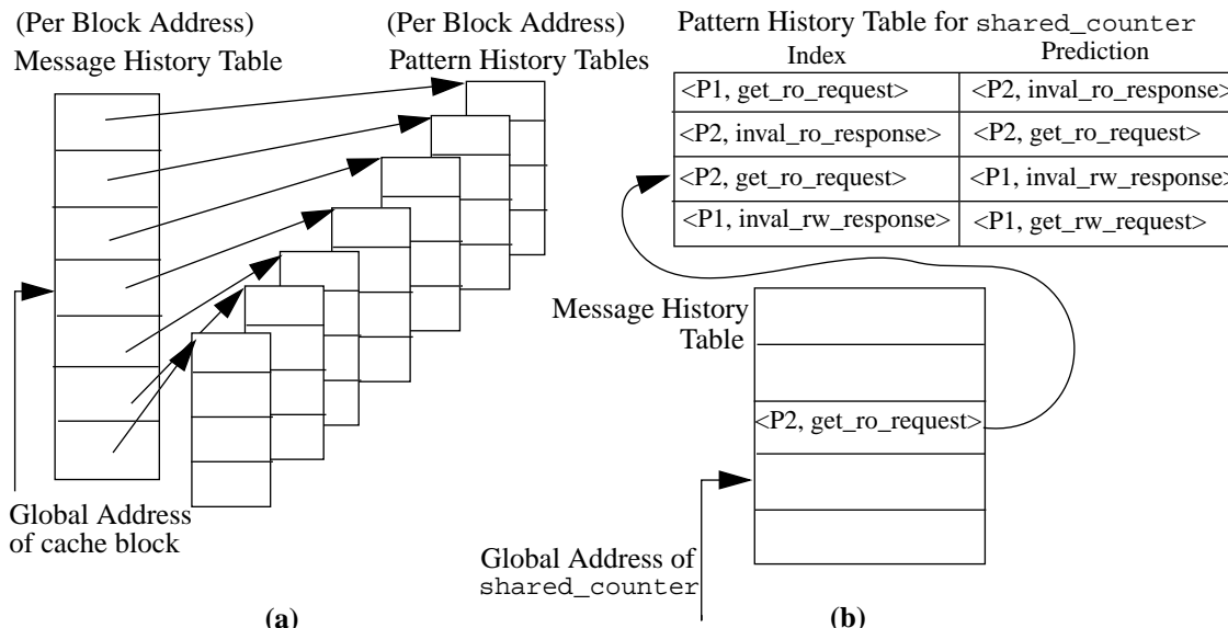
Figure 6-3. Cosmos' structure. (a) shows the logical structure the Cosmos coherence message predictor and (b) shows an example of how the message and pattern history tables for a directory may look like for the shared_counter in Figure 6-2. In this example, I assume that the last message received by the directory is a get_ro_request from the consumer (denoted as P2). So, Cosmos will predict the next message to be an inval_rw_response from the producer (denoted as P1).
