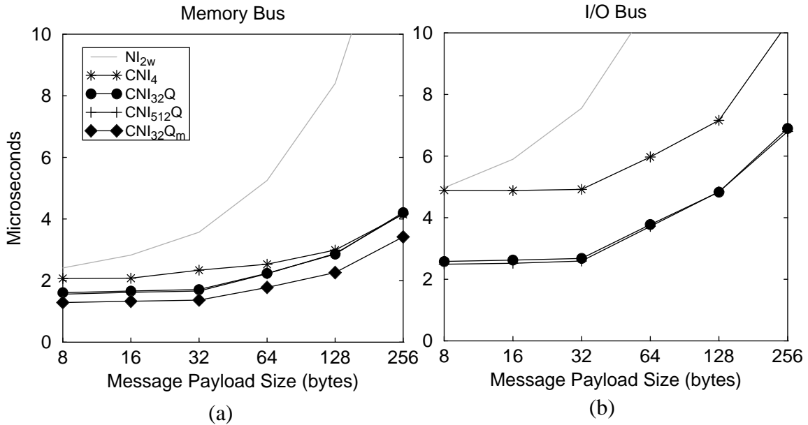
Figure 4-1. Process-to-process round-trip message latency. This figure shows the process-to-process round-trip message latency in microseconds (vertical axis) for different message sizes (horizontal axis). (a) shows the round-trip message latency for NI 2w , CNI 4 , CNI 32Q , CNI 512Q , and CNI 32Q m on the memory bus. (b) shows the same (except CNI 32Q m ) on the I/O bus.
