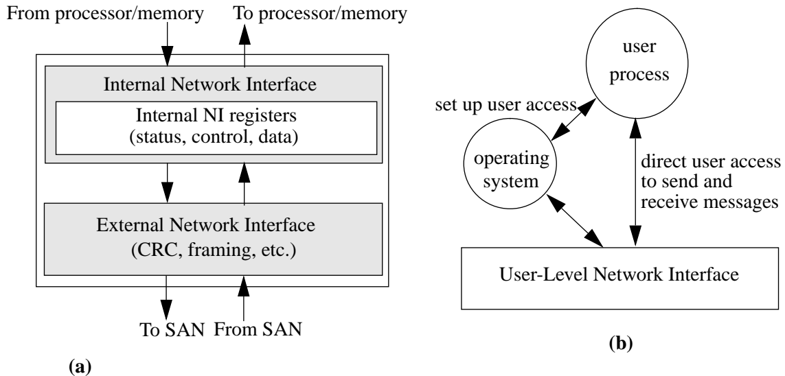
Figure 1-2. High-level views of an NI. (a) shows the building blocks of an NI. (b) shows how a user process can logically access an NI.
