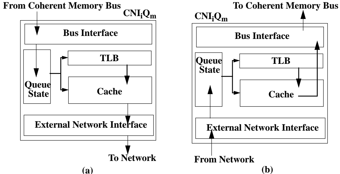
Figure 3-6. Logical datapath through multiprogrammed CNI_iQ_m device. This figure shows the logical path through followed by a message for a message send (a) and message receive (b) for a multiprogrammed CNI_iQ_m device.
