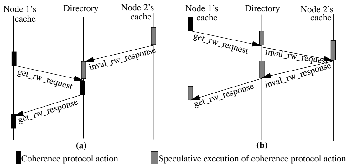
Figure 6-4. Two examples of using prediction to accelerate coherence protocols. (a) shows a protocol in which protocol actions are accelerated in anticipation of Node 1's write miss. (b) shows a protocol that predicts incoming coherence messages, updates protocol state, generates (but does not send) messages speculatively, and commits protocol state and messages only if the predicted message arrives.
