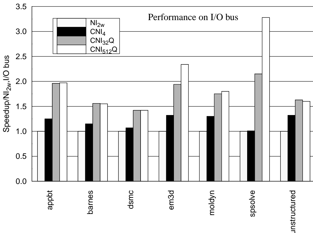
Figure 4-5. CNIs' performance on the I/O bus. This figure compares the performance of NI 2w , CNI 4 , CNI 32Q , and CNI 512Q on the I/O bus for seven macrobenchmarks. The vertical axis shows the speedup of each of the NIs over NI 2w .
