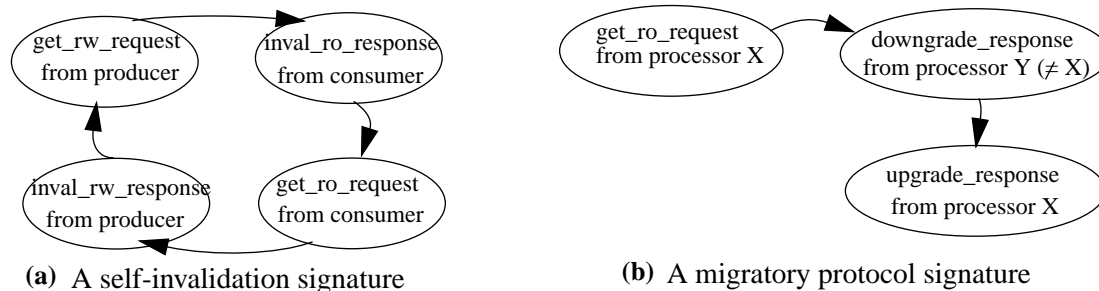
Figure 6-9. Signatures for dynamic self-invalidation and migratory protocols. The downgrade_response , not shown in Table 6.1, is a response to a downgrade_request sent by the directory. On receiving a downgrade_request for a block, a cache must change the block from exclusive to shared state.
