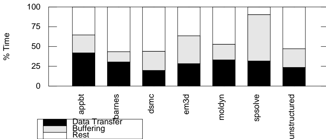
Figure 5-1. Impact of data transfer and buffering. This figure demonstrates the impact of data transfer and buffering on the performance of a memory bus NI for seven parallel scientific applications. For these measurements, I use a CM-5-like network interface and number of flow control buffers equal to 1. See Section 5.3 and Section 5.4 for a description of my CM-5-like NI, my flow control scheme, and the applications.
