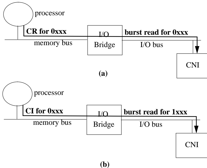
Figure 3-5. Illustration of shadow address with a CNI on the I/O bus. (a) a processor read miss (CR = coherent read) for the address 0xxx is translated by the bridge to a burst read for 0xxx on the I/O bus. (b) shows that a CI (coherent invalidate) signal for 0xxx is translated to a burst read for the shadow address 1xxx. The CNI interprets a read for 1xxx as an invalidation signal for 0xxx.
