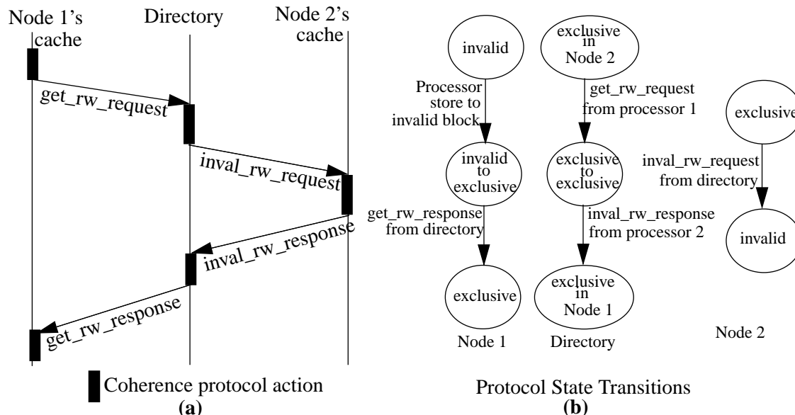
Figure 6-1. Basic structure of a directory protocol. (a) shows message exchange between a directory and two caches and (b) shows the corresponding state transitions. Table 6.1 contains an explanation of the coherence message types. Initially, processor 2 has an exclusive copy of a cache block. Processor 1 issues a store to the block. This invokes the coherence protocol, which sends a message to the directory. The directory examines its state and sends a message to processor 2 requesting it to return the block to the directory and invalidate its copy of the block. When it receives the block from processor 2, it forwards it to processor 1, which marks the cache block as exclusive in processor 1. The states “invalid to exclusive” and “exclusive to exclusive” represent transition states.
