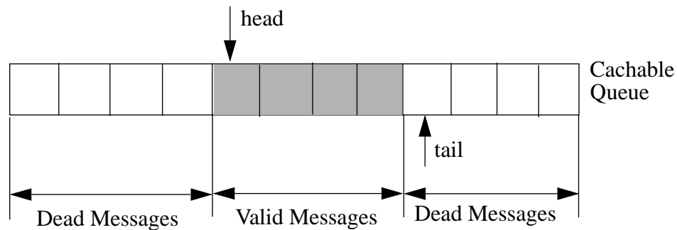
Figure 3-4. Dead message elimination. A simple comparison of the head and tail pointer shows messages that are already consumed by the receiver.
