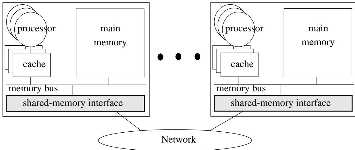
Figure 1-3. A shared-memory multiprocessor.
