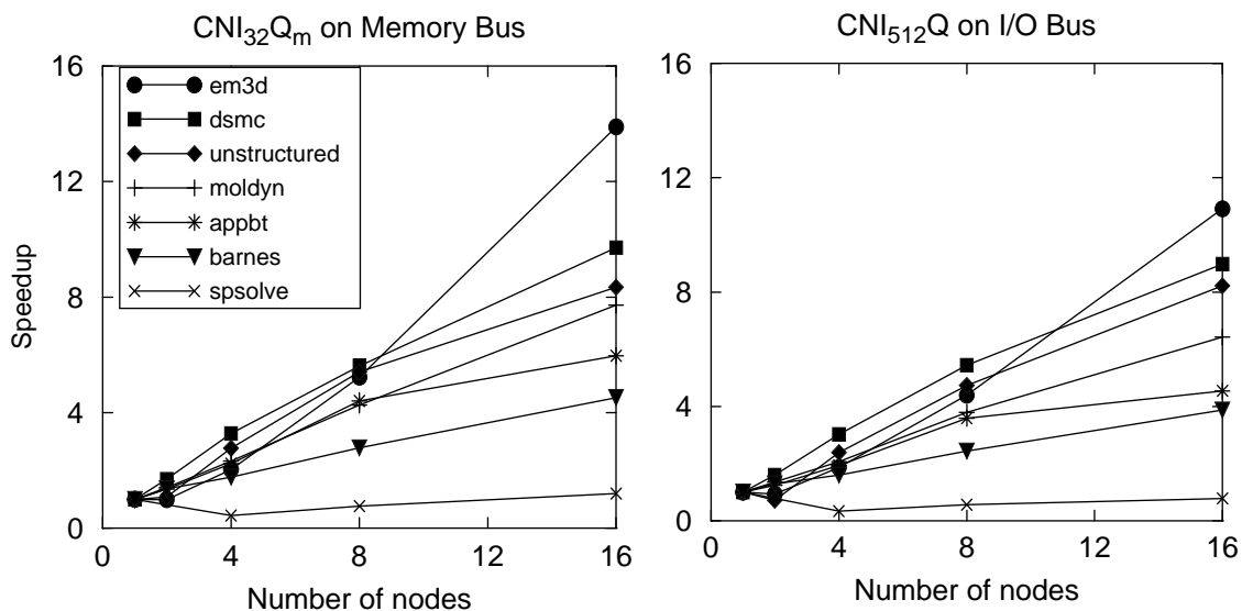
Figure 4-8. Macrobenchmark speedup. This figure shows the speedup of the seven macrobenchmarks with CNI 32 Q m on the memory bus and CNI 512 Q on the I/O bus. These NIs perform the best on the respective buses.
