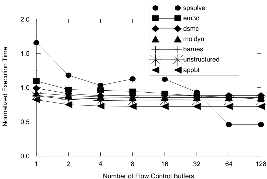
Figure 5-3. Comparison of execution of a single-cycle NI_{2w} with CNI_{32}Q_m . The vertical axis is normalized to the CNI_{32}Q_m on the memory bus. CNI_{32}Q_m is independent of flow control buffering because it provides plentiful buffering in main memory.
