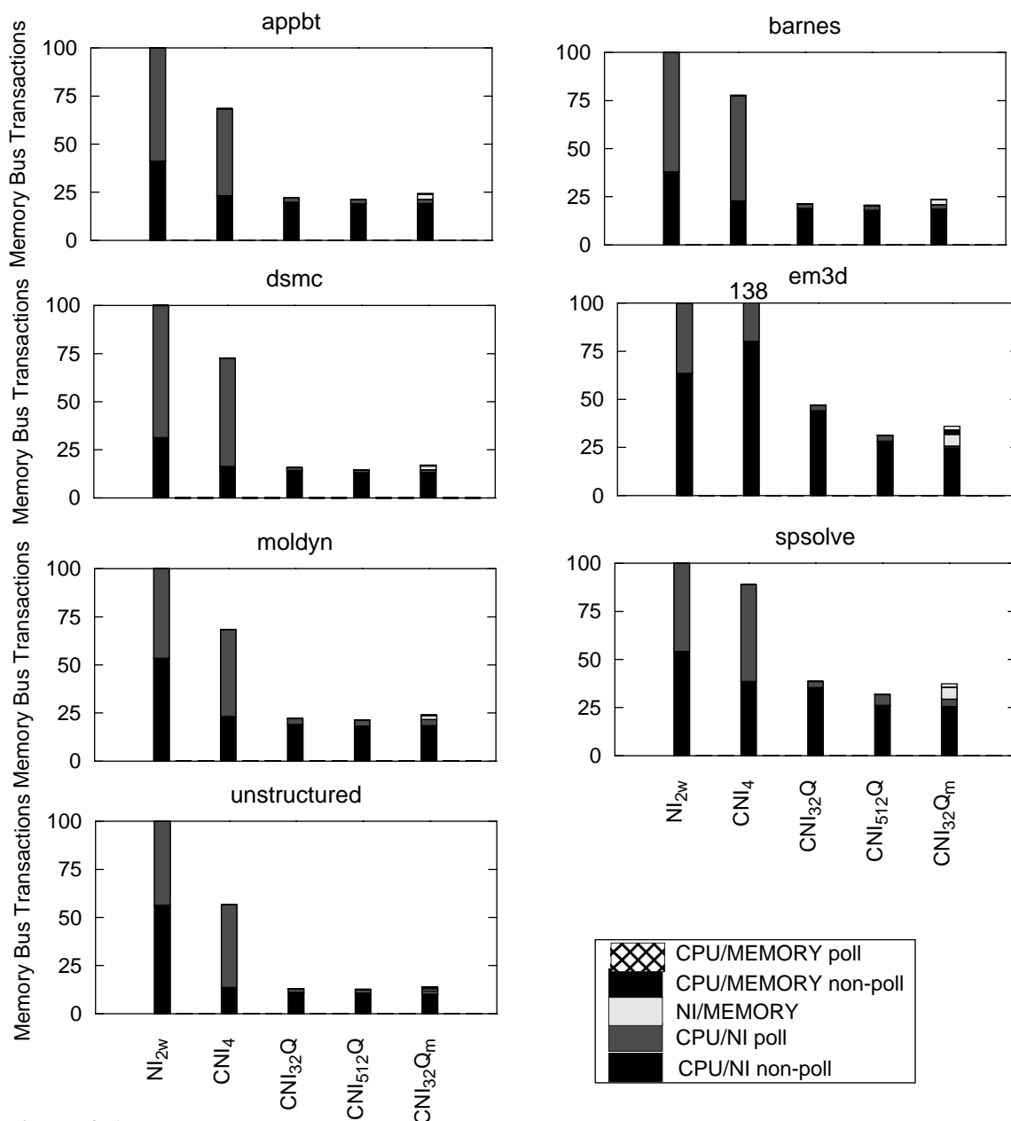
Figure 4-6. Breakdown of memory bus transactions for five memory bus NIs. This figure shows the breakdown of memory bus transactions for five memory bus NIs totalled across all 16 nodes. The notation X/Y denotes that the transaction happened between modules X and Y on the memory bus. For NI 2w and CNI 4 , poll denotes transactions corresponding to a processor's polls to the send and receive status registers. For CQ-based CNIs, poll denotes the processor's cache misses for cache blocks that return without valid data and the processor's polls for the send status register, which is uncached in these CNI implementations. Non-poll denotes all NI-related transactions other than polls. CNI 4 with em3d shows a slight anomaly because node 15 became a hot spot due to accidental differences in global memory allocation. However, this appears to have only significantly affected the bus transaction count, and not the total execution time of CNI 4 .
