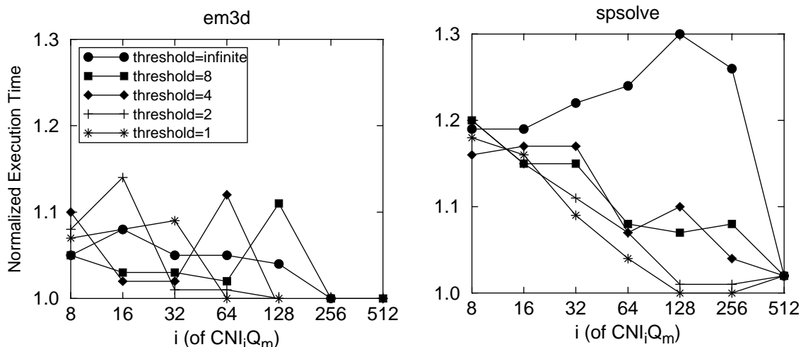
Figure 4-7. CNI_i Q_m cache size variation. This figure shows the effect of varying CNI_i Q_m 's cache size, i.e. “ i ”, and the dead message elimination threshold described in Section 3.3.2. Each graph is normalized to the execution time of CNI_{128} Q_m with threshold = 1. An infinite threshold indicates no dead message elimination optimization.
