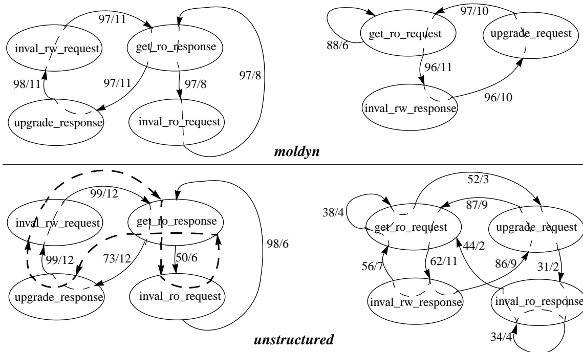
Figure 6-6. Dominant (incoming) message signatures for moldyn and unstructured . See caption of Figure 6-5 for an explanation of the figure. I show unstructured 's second dominant message signature (at the cache) using bold and dashed lines.
