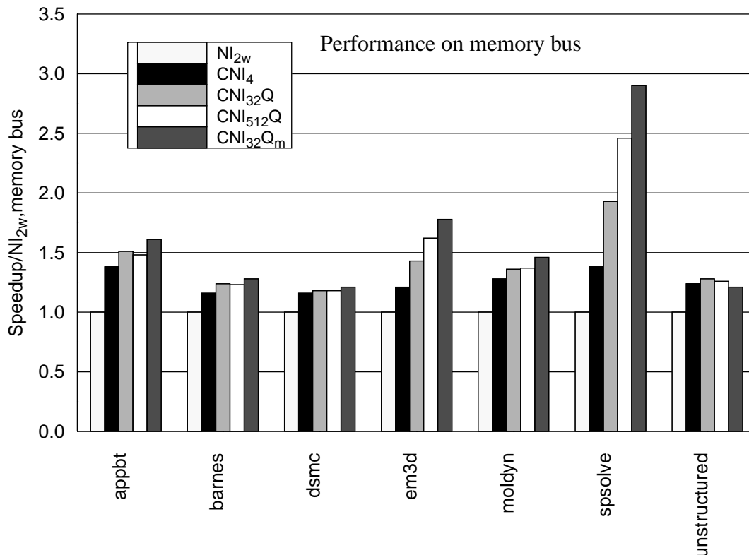
Figure 4-4. CNIs' performance on the memory bus. This figure compares the performance of NI 2w , CNI 4 , CNI 32Q , CNI 512Q , and CNI 32Q m on the memory bus for seven macrobenchmarks. The vertical axis shows the speedup of each of the NIs over NI 2w .
