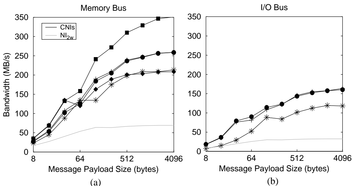
Figure 4-3. Process-to-process message bandwidth. This figure shows the process-to-process message bandwidth in megabytes per second (vertical axis) for different message sizes (horizontal axis). (a) shows the process-to-process message bandwidth for NI 2w , CNI 4 , CNI 32Q , CNI 512Q , CNI 32Q m , and CNI 32Q m with send throttling. (b) shows the same (except the CNI 32Q m graphs). CNI Legend: ■ = CNI 32Q m +send throttle, ◆ = CNI 32Q m , + = CNI 512Q , ● = CNI 32Q , * = CNI 4 .
