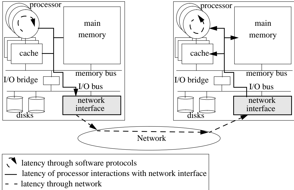
Figure 1-1. Three components of message latency.
