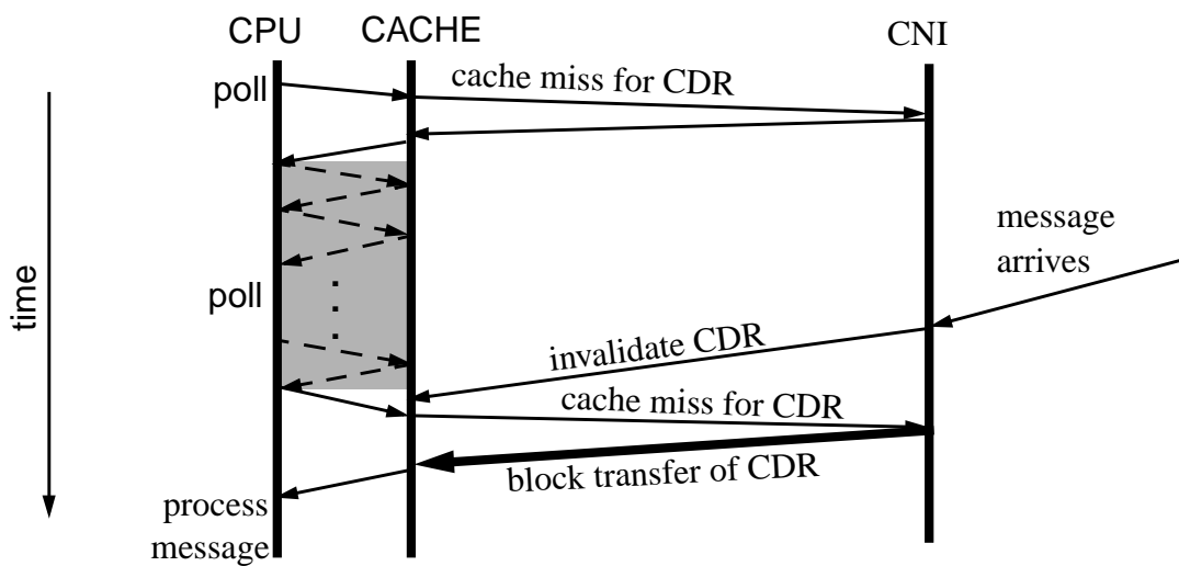
Figure 3-1. CDR Transfer Example. This figure shows CDR transfers between the CPU, CPU's cache, and a CNI, assuming write-allocate caches kept consistent by a MOESI write-invalidate coherence protocol [123]. Initially, the CPU polls a CDR to check the presence of a message. Assume this incurs a cache miss. This cache miss is satisfied by the CNI (instead of main memory), which indicates the absence of any message in the CNI. The CPU's subsequent polls to the CDR block (shaded region) is satisfied directly from its cache. Finally, a message arrives, which prompts the CNI to invalidate the CDR block in the CPU's cache following the standard coherence protocol supported by the memory bus. The subsequent cache miss for the CDR block brings in the new CNI status and the first few words of the message in one block.
