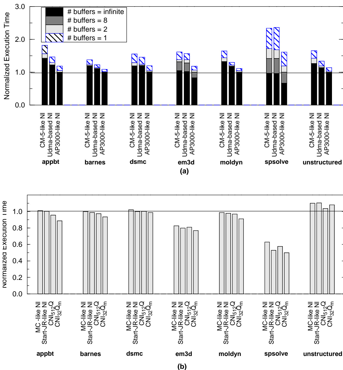
Figure 5-2. Comparison of execution time of seven NIs. Both (a) and (b) are normalized to the AP3000-like NI with number of flow control buffers = 8. # buffers denotes the number of flow control buffers. (a) compares the performance of my three fifo-based NIs for different levels of flow control buffering. The black shade represents the execution time with infinite flow control buffering. Lighter shades represent the incremental execution time penalty for three flow control buffering levels (8, 2, and 1). (b) compares the performance of four coherent network interfaces with number of flow control buffers = 2. However, because these NIs themselves provide plentiful buffering, their performance is largely insensitive to the number of flow control buffers. MC-like NI denotes the Memory Channel-like NI.
