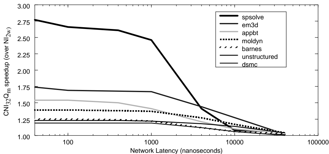
Figure 4-9. Impact of Network Latency.
