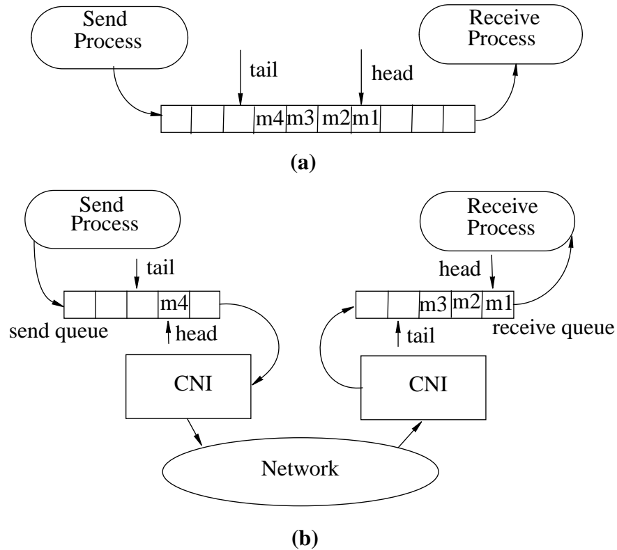
Figure 3-2. Cachable Queues. (a) Local Cachable Queue (b) Remote Cachable Queue. m_1 , m_2 , m_3 , and m_4 denote valid messages sent by the Send Process to the Receive Process.
