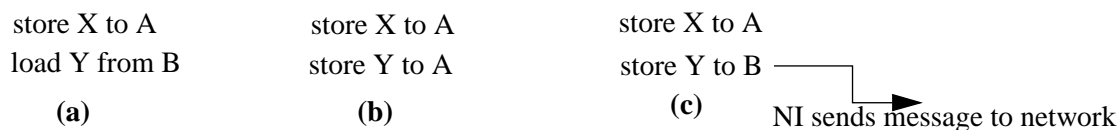
Figure 2-3. Three examples of side-effects in existing NI designs. The instructions shown in this figure are uncached loads and stores to ULNI registers memory-mapped to virtual addresses A and B. (a) shows that the store-load pair must be strictly in order for some NIs to work correctly (e.g., Princeton UDMA initiation), even though the instructions appear unrelated to the processor. (b) shows two consecutive stores to the same address must occur in order (e.g., TMC CM-5 NI). (c) extends (b) to show that the second store (in the general case, the “n”th store) can trigger an action in the NI, such as sending a message into the network. (a) and (b) have the side-effects that a previous store determines implicitly the next uncached load or store a NI expects. (c) has the side-effect of sending a message on a store.
